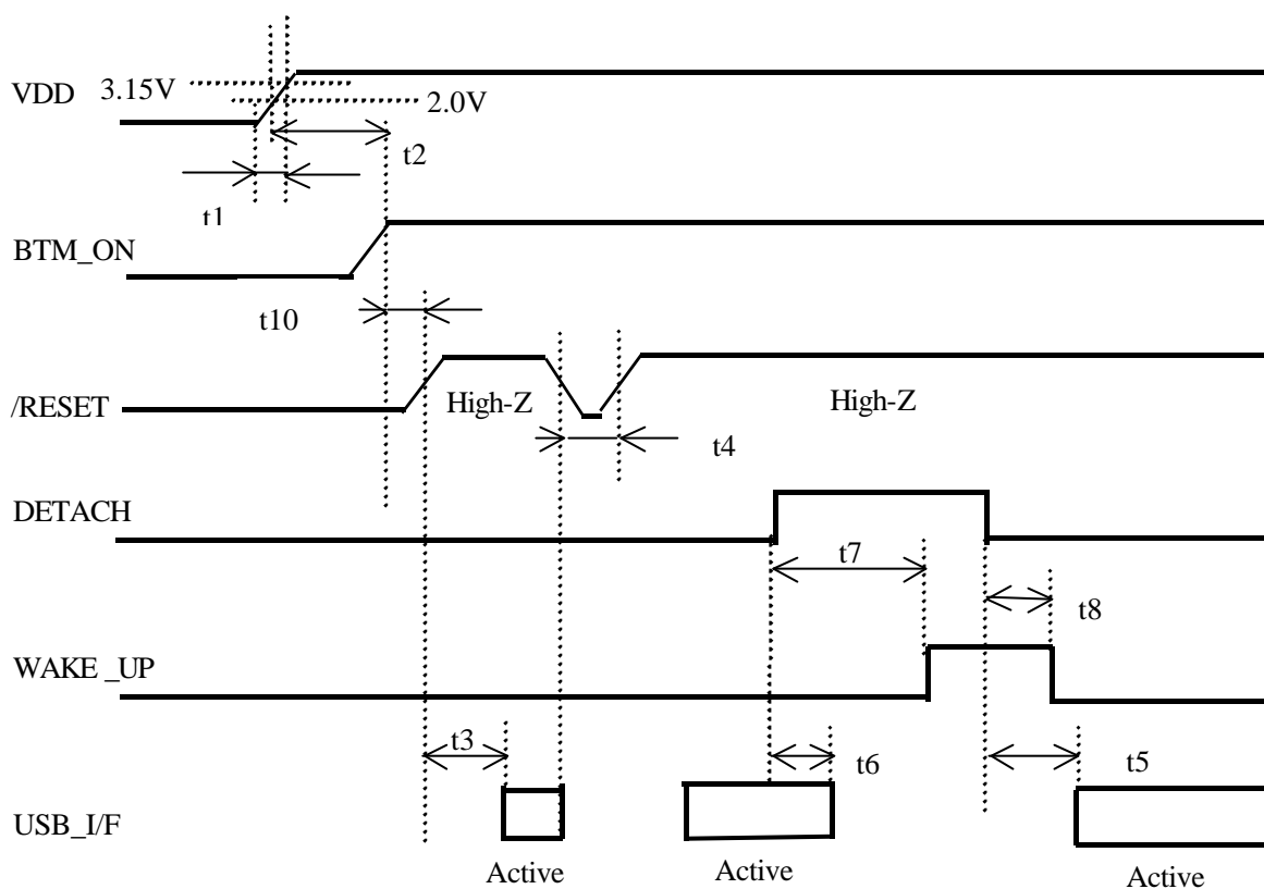
Timing Diagram for Power Up Sequence
